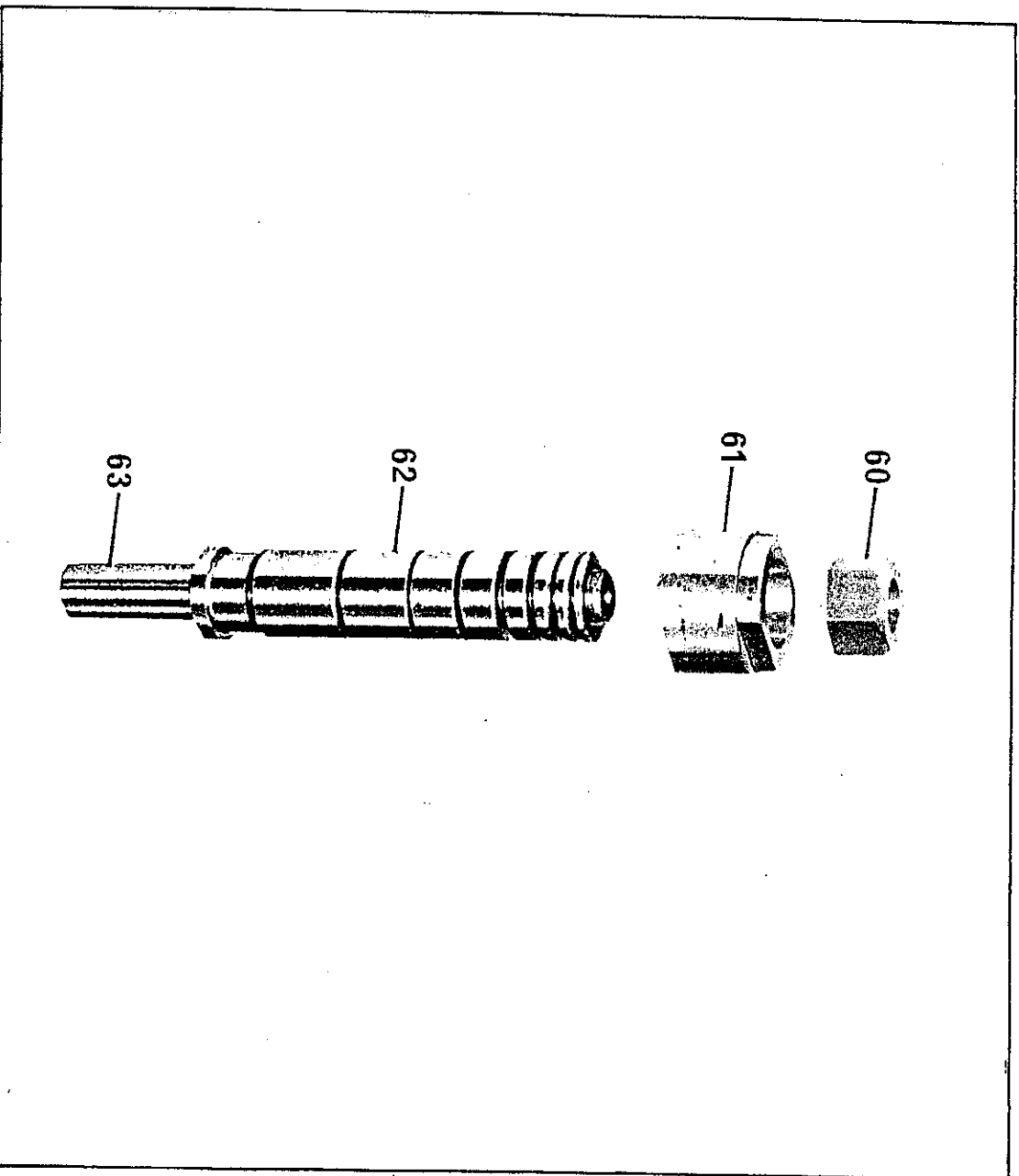
WORK SPINDLE ASSEMBLY
