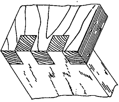
BOX JOINT
