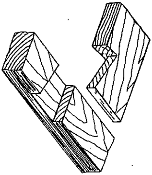
DOVETAIL HALF LAP (ONE SIDE ONLY)
