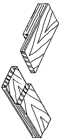
END HALF LAP
