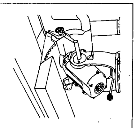
BEVEL RIPPING.
