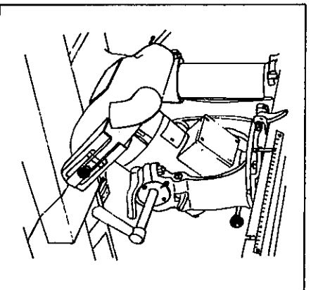
BEVEL CROSSCUTTING.
