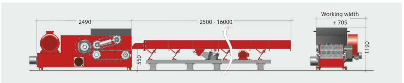
Rotor Version 5
